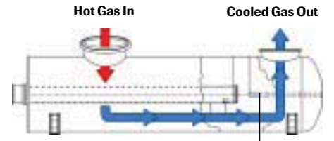
Mesh Demister
