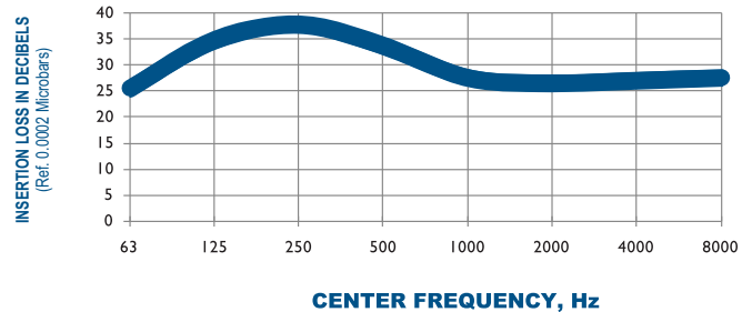
TYPICAL ATTENUATION CURVE A202-5100 OCTAVE BAND
