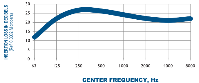
TYPICAL ATTENUATION CURVE H9-4 OCTAVE BAND
