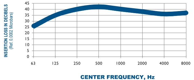
TYPICAL ATTENUATION CURVE 501-C1-5100 OCTAVE BAND
