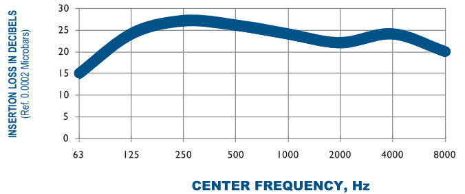
TYPICAL ATTENUATION CURVE 301-6100 OCTAVE BAND
