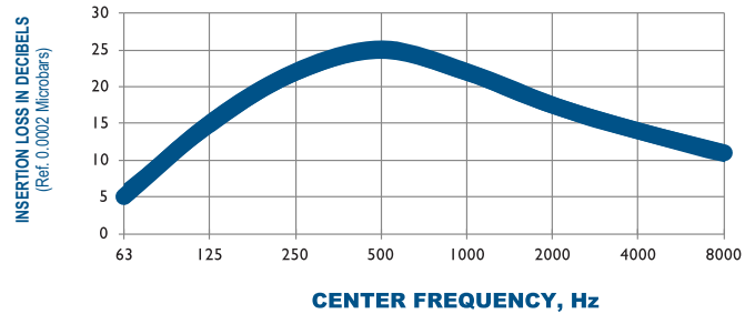
TYPICAL ATTENUATION CURVE A203-2100 OCTAVE BAND
