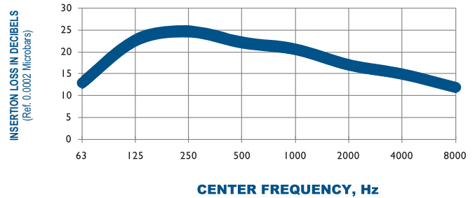
TYPICAL ATTENUATION CURVE A202-2100 OCTAVE BAND
