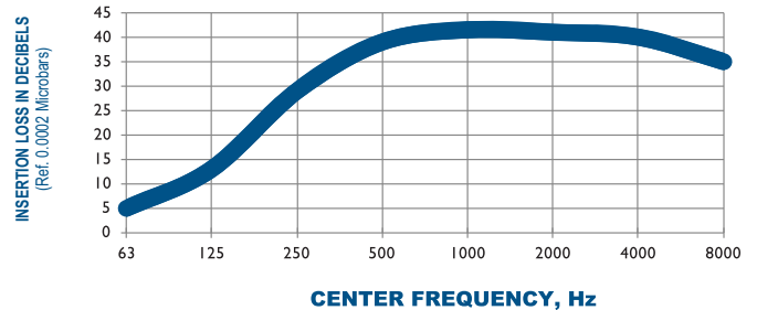
TYPICAL ATTENUATION CURVE A205-5100 OCTAVE BAND
