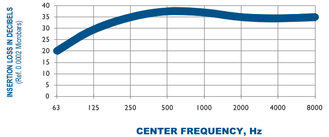
TYPICAL ATTENUATION CURVE H3-5 OCTAVE BAND
