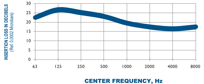
TYPICAL ATTENUATION CURVE A201-4100 OCTAVE BAND
