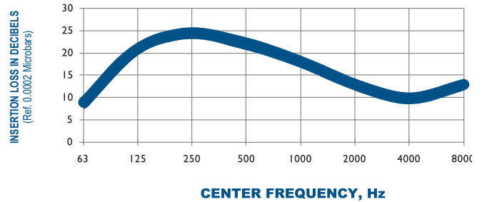
TYPICAL ATTENUATION CURVE 201-1100 OCTAVE BAND
