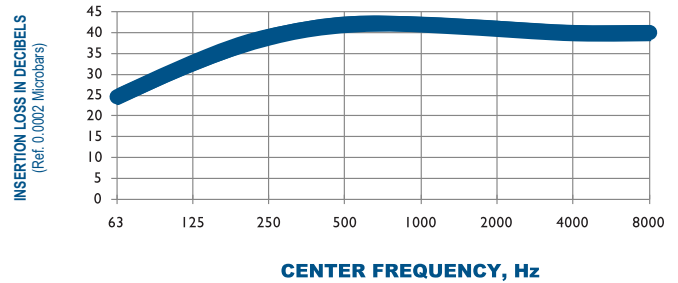
TYPICAL ATTENUATION CURVE H1-6 OCTAVE BAND
