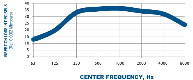
TYPICAL ATTENUATION CURVE H3-4 OCTAVE BAND
