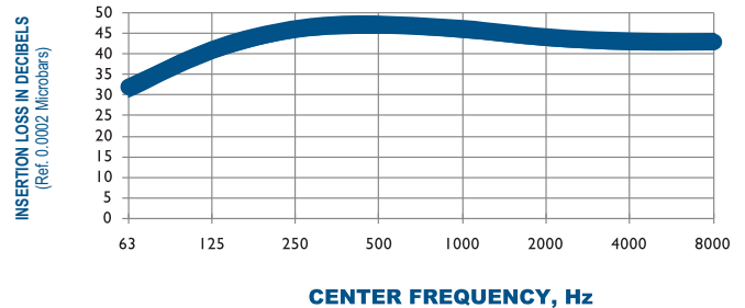
TYPICAL ATTENUATION CURVE 501-C2-6100 OCTAVE BAND
