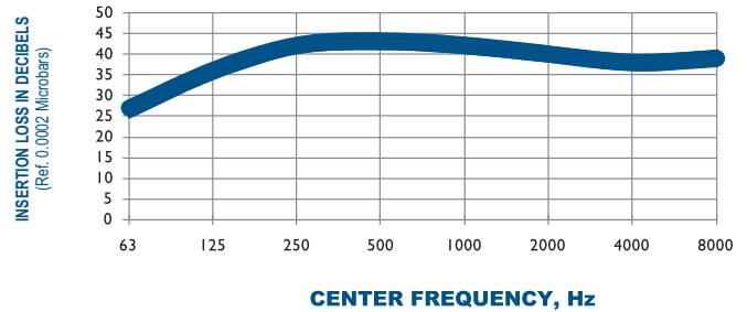
TYPICAL ATTENUATION CURVE 501-C2-5100 OCTAVE BAND
