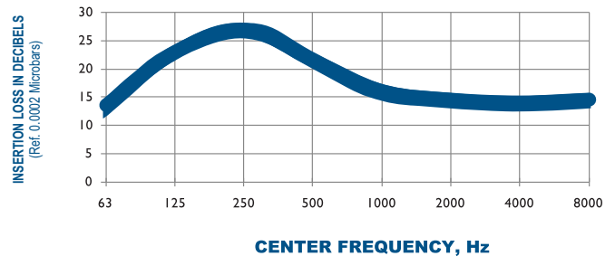
TYPICAL ATTENUATION CURVE A201-2100 OCTAVE BAND
