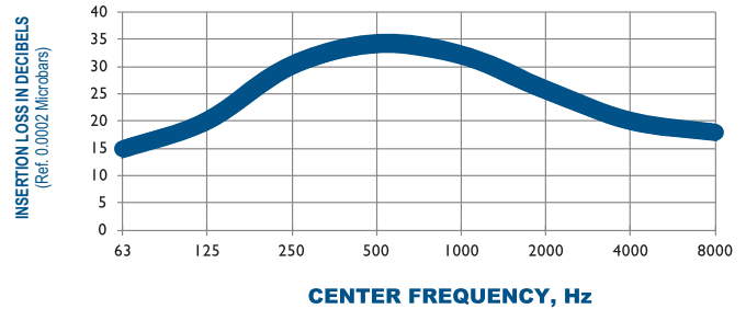
TYPICAL ATTENUATION CURVE A203-4100 OCTAVE BAND
