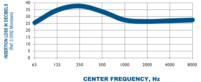
TYPICAL ATTENUATION CURVE A201-5100 OCTAVE BAND
