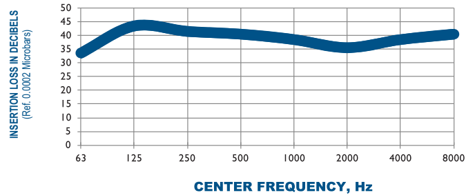
TYPICAL ATTENUATION CURVE A201-7100 OCTAVE BAND
