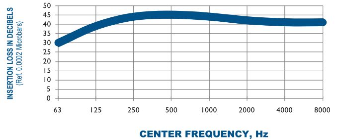
TYPICAL ATTENUATION CURVE 501-C1-6100 OCTAVE BAND
