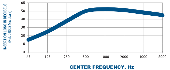
TYPICAL ATTENUATION CURVE A205-6100 OCTAVE BAND
