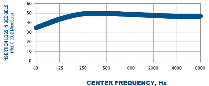
TYPICAL ATTENUATION CURVE 501-C1-7100 OCTAVE BAND
