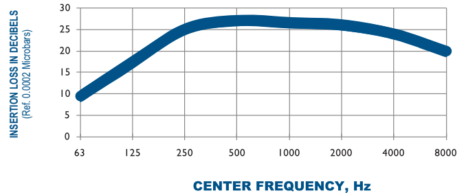
TYPICAL ATTENUATION CURVE H5-4 OCTAVE BAND
