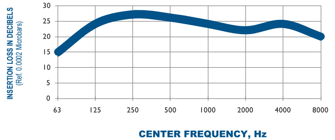
TYPICAL ATTENUATION CURVE 301-4100 OCTAVE BAND
