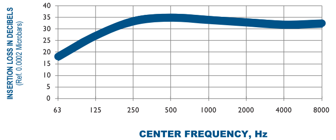
TYPICAL ATTENUATION CURVE H5-5 OCTAVE BAND
