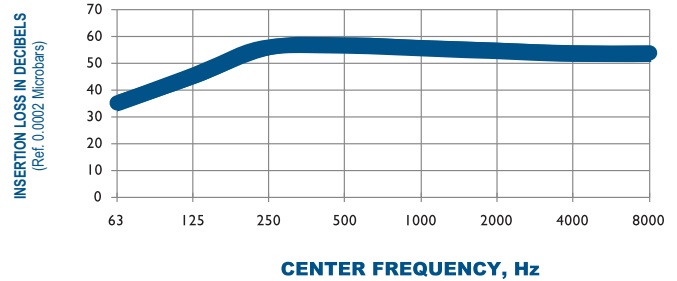
TYPICAL ATTENUATION CURVE 501-C2-7100 OCTAVE BAND
