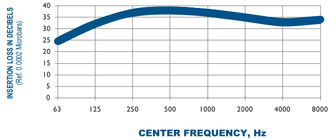
TYPICAL ATTENUATION CURVE 501-5200 OCTAVE BAND
