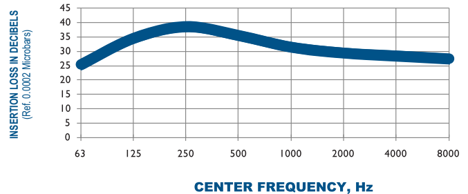
TYPICAL ATTENUATION CURVE A201-5600 OCTAVE BAND
