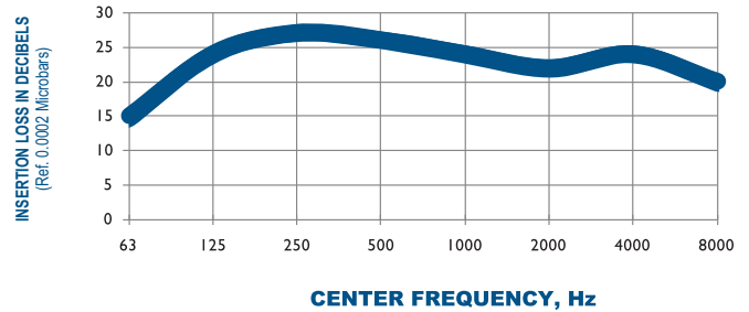
TYPICAL ATTENUATION CURVE 301-5100 OCTAVE BAND
