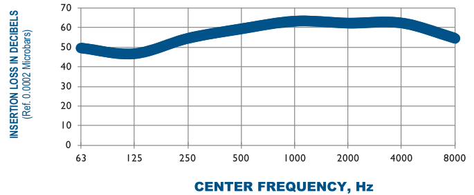
TYPICAL ATTENUATION CURVE A201-8100 OCTAVE BAND
