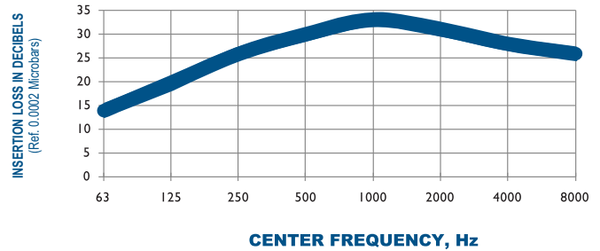
TYPICAL ATTENUATION CURVE H9-5 OCTAVE BAND
