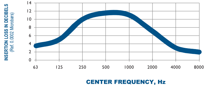
TYPICAL ATTENUATION CURVE 202-1100 OCTAVE BAND
