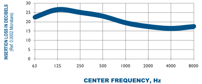
TYPICAL ATTENUATION CURVE A202-4100 OCTAVE BAND
