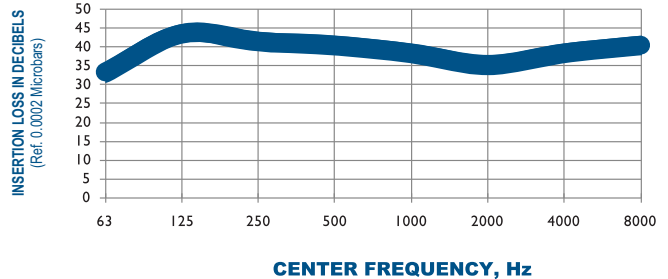
TYPICAL ATTENUATION CURVE A202-6100 OCTAVE BAND
