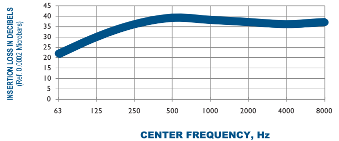
TYPICAL ATTENUATION CURVE H1-5 OCTAVE BAND
