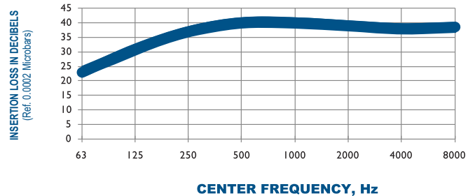
TYPICAL ATTENUATION CURVE H3-6 OCTAVE BAND
