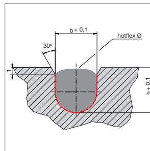
Round groove geometry
