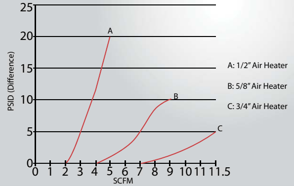
Input / Output Airflow Test
