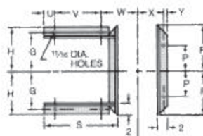
FOUNDATION PLAN
