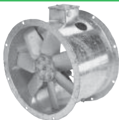
AEROFOIL ADJUSTABLE PITCH FAN Available in 21 Sizes 12" to 110". CFM from 500 to 350,000. Static pressures to 15" W.G. Multiple stages available for higher pressures. Request Bulletin IJMA60-99..
