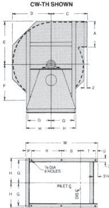
FOUNDATION PLAN ALL DISCHARGES EXCEPT DB
