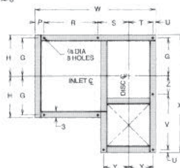
DOWNBLAST DISCHARGE FOUNDATION PLAN CW-DB SHOWN CCW-DB IS MIRROR IMAGE
