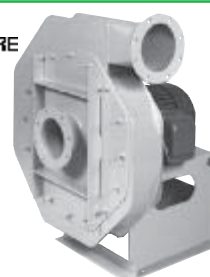
9 Sizes from 400 to 8,000 CFM. 4 wheel types. Pressures to 75" W.G. Request Bulletin VP-0404.
