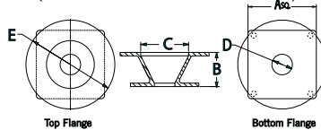
Machine Mount Adapter (Included with MM mode[s])
