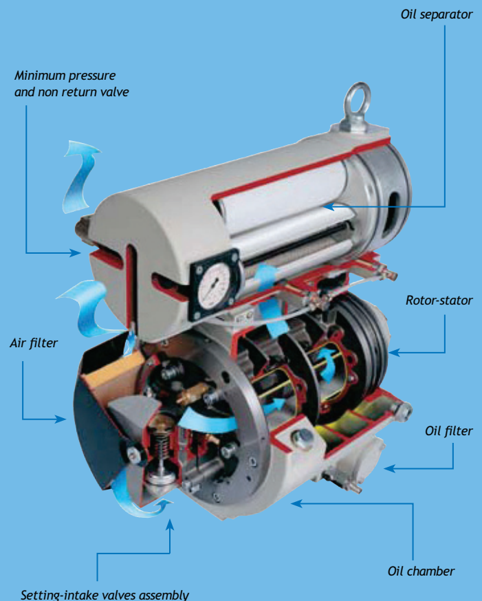
Figure 3: Airend Construction
